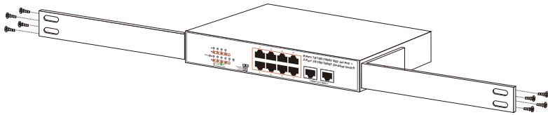
Attaching the Brackets to the DT10-2G-8GP+
