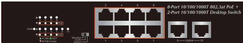
DT10-2G-8GP+ Switch Front Panel
