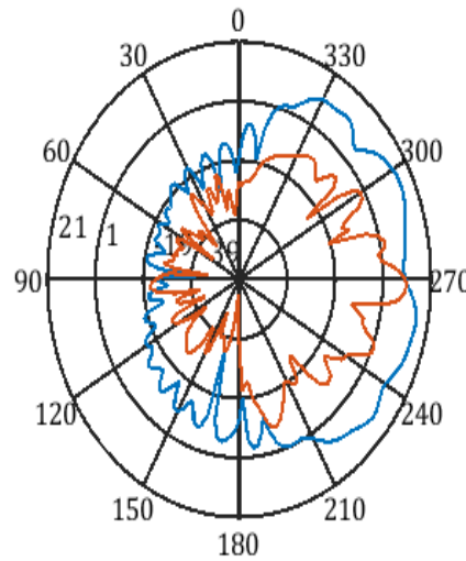
f=6300MHz, Co@2-cuts
