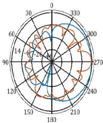
f=2300MHz, Co@2-cuts
