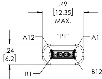
USB 3.1 PLUG SERIES "C" GOLD PLATED PINS
