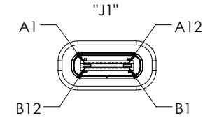
USB 3.1 RECEPTACLE SERIES "C" GOLD PLATED PINS
