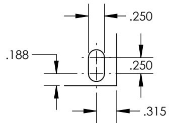
DETAIL A SCALE 2 : 3
