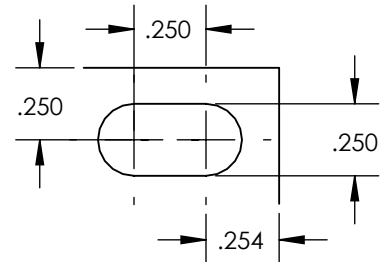
DETAIL A SCALE 3 : 2
