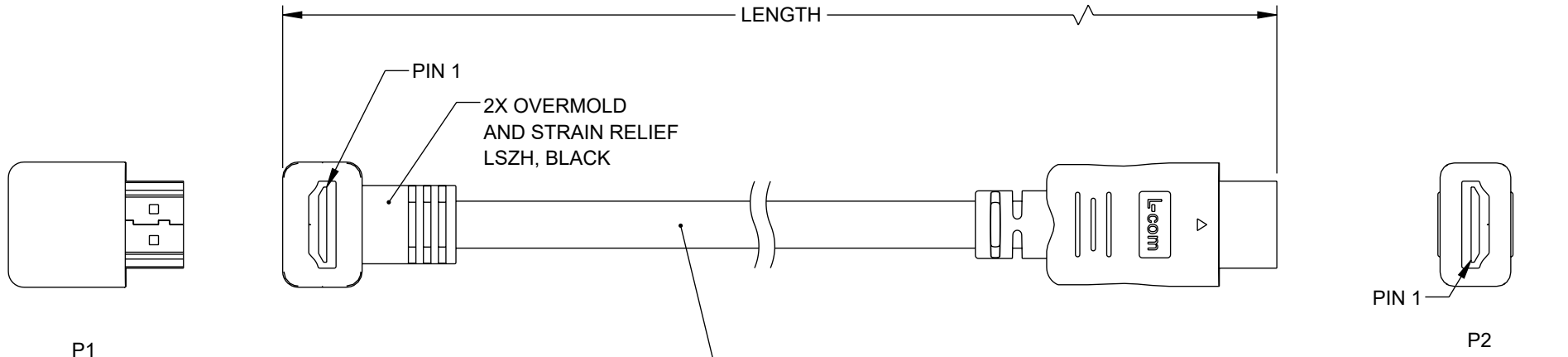
P1 HDMI 2.1 MALE UP ANGLE CONNECTOR
