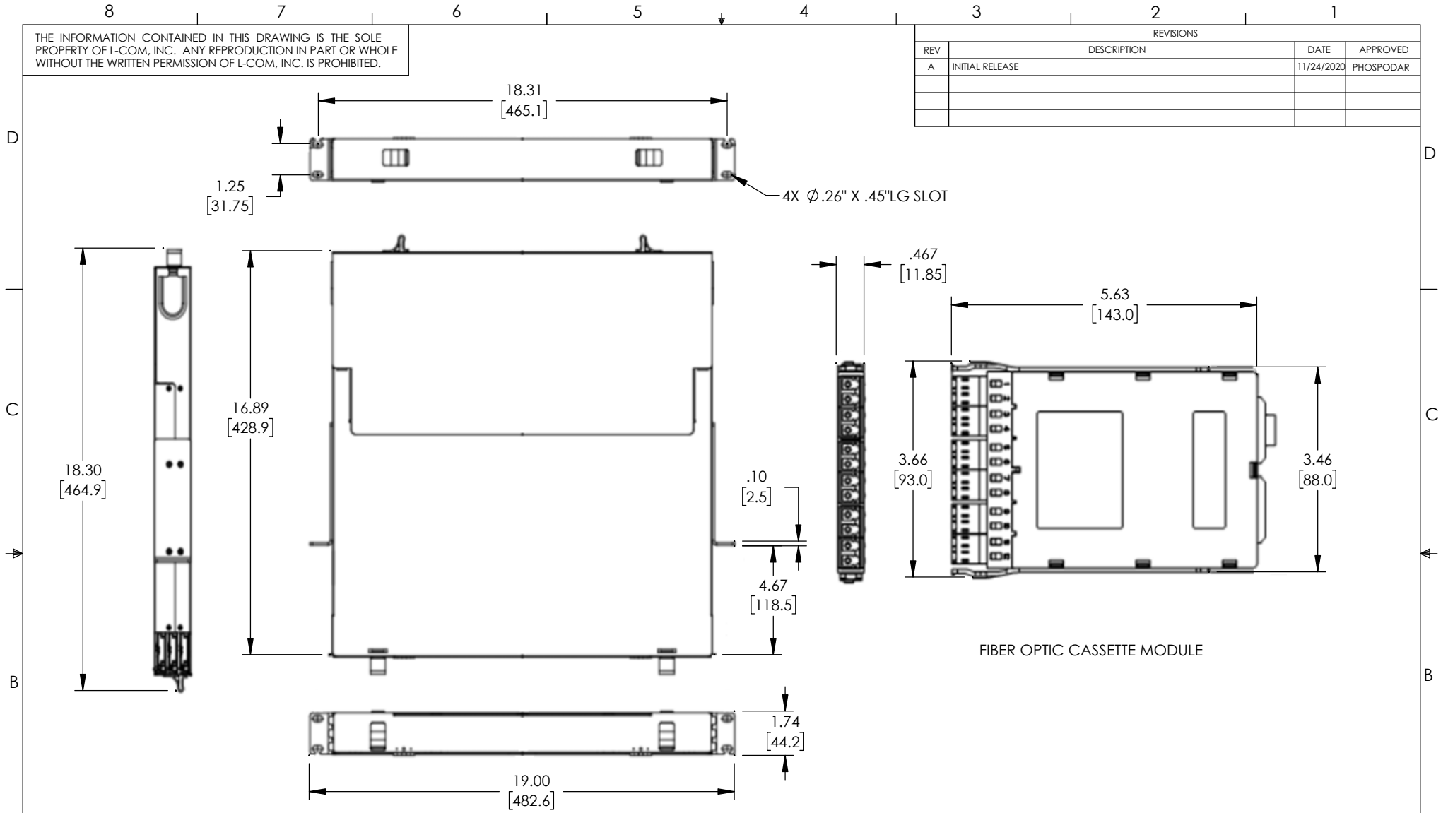
FIBER OPTIC PATCH PANEL
