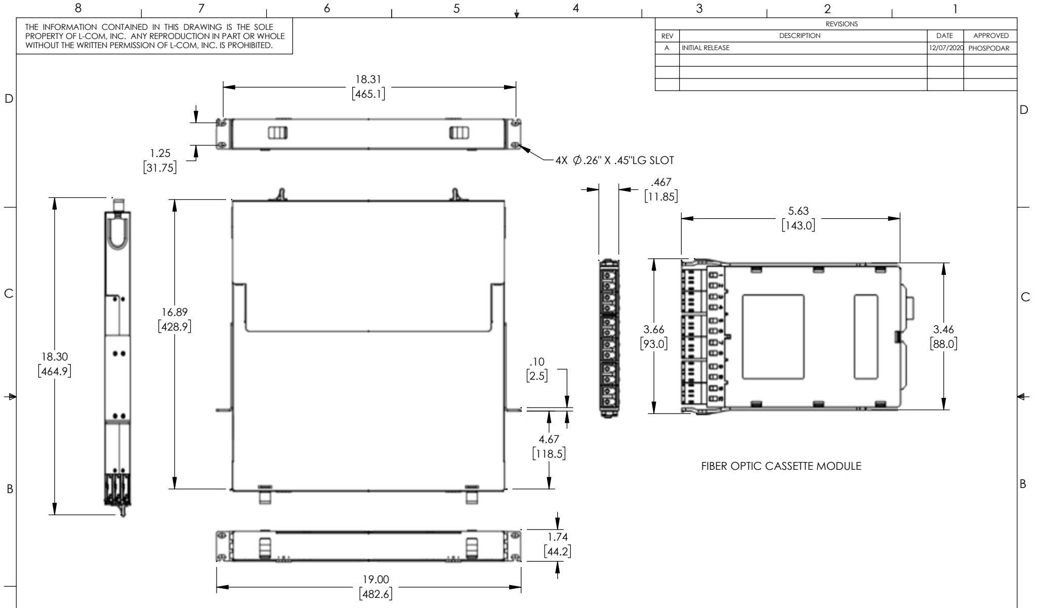
FIBER OPTIC PATCH PANEL
