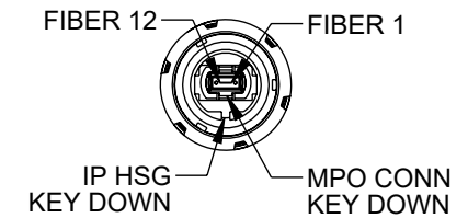
VIEW B-B
