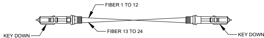
24 FIBER MPO POLARITY: METHOD B, KEY DOWN-KEY DOWN
