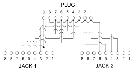
WIRING DIAGRAM LABEL
