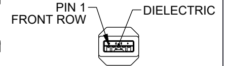
"P2" USB 3.0 TYPE A PLUG CONTACTS 30μ" GOLD
