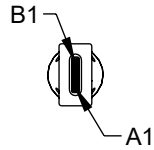
"P1" USB3.0 TYPE C PLUG CONTACTS 30μ" GOLD
