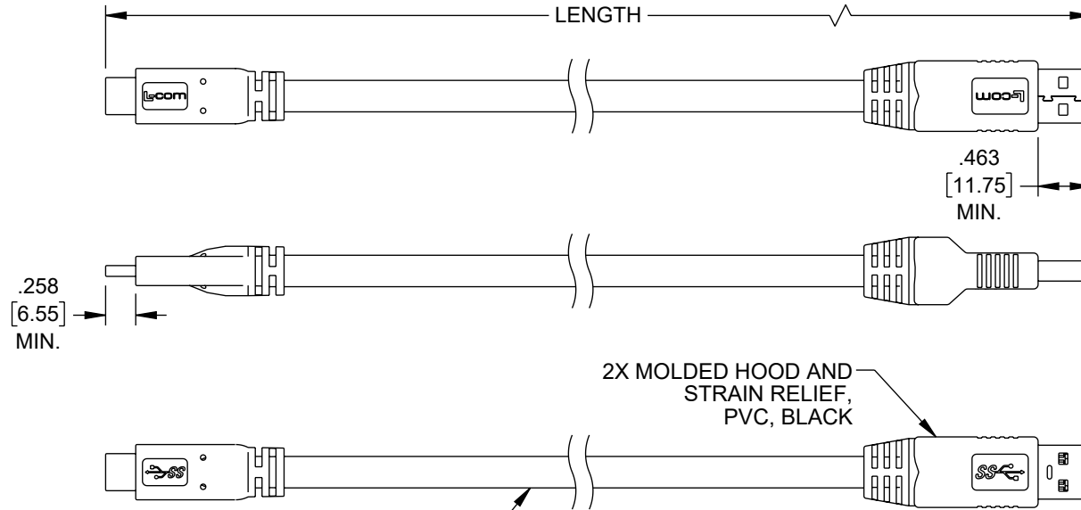
"P1" USB3.0 TYPE C PLUG CONTACTS 30μ" GOLD
