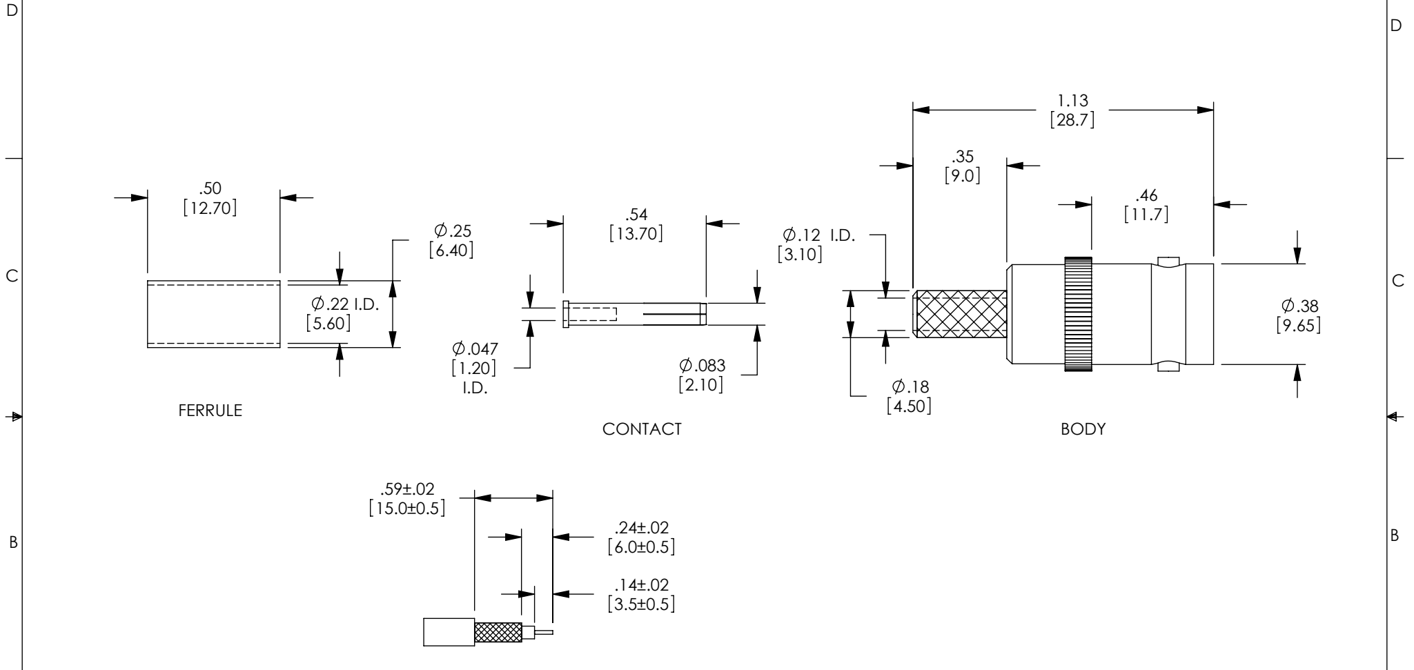
RECOMMENDED CABLE STRIPPING
