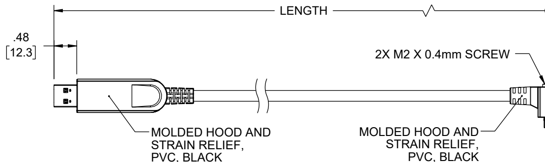
"P2" USB 3.2 MICRO-B 90° PLUG
