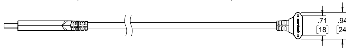
"P2" USB 3.2 MICRO-B 90° PLUG
