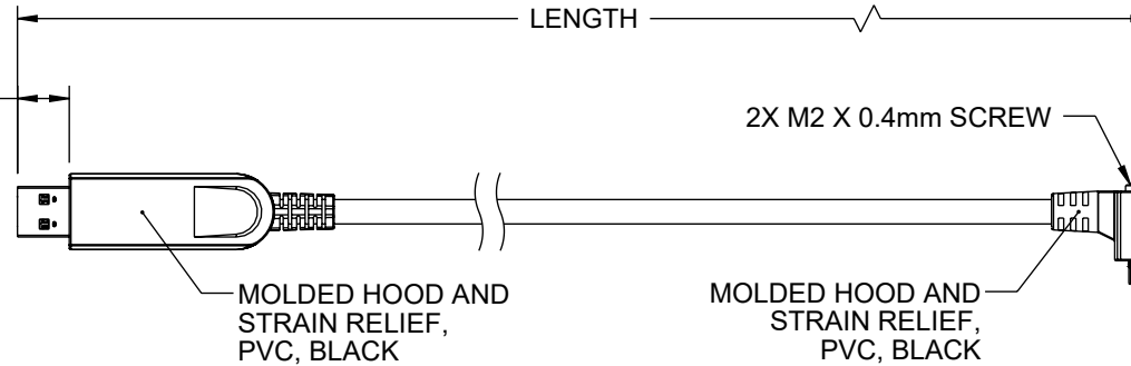
"P2" USB 3.2 MICRO-B 90° PLUG
